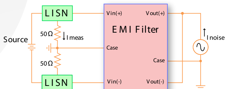
Figure B: Common-Mode Current Attenuation, I_{meas} / I_{noise}
