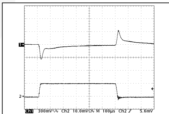
Figure 12: Output voltage response to step-change in load current (0%-50%-0% of I_{out(max)} ). Load cap: 1 \mu F ceramic cap and 10 \mu F, 100 m \Omega ESR tantalum cap. Ch 1: Vout (300mV/div). Ch 2: Iout (10A/div).
