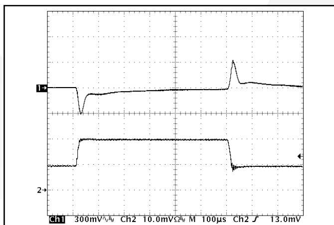
Figure 11: Output voltage response to step-change in load current (50%-100%-50% of I_{out(max)} ). Load cap: 1 \mu F ceramic cap and 10 \mu F, 100 m \Omega ESR tantalum cap. Ch 1: Vout (300mV/div). Ch 2: Iout (10A/div).
