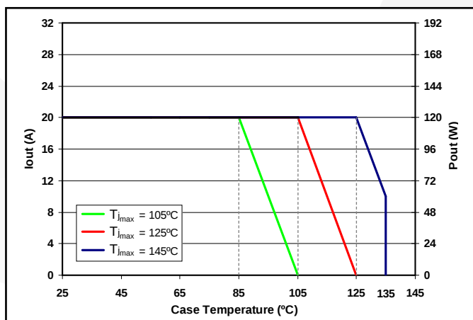
Figure 5: Output Current / Output Power derating curve as a function of T_{CASE} and the Maximum desired power MOSFET junction temperature at V_{in} = 28\text{V} (see Note 14).
