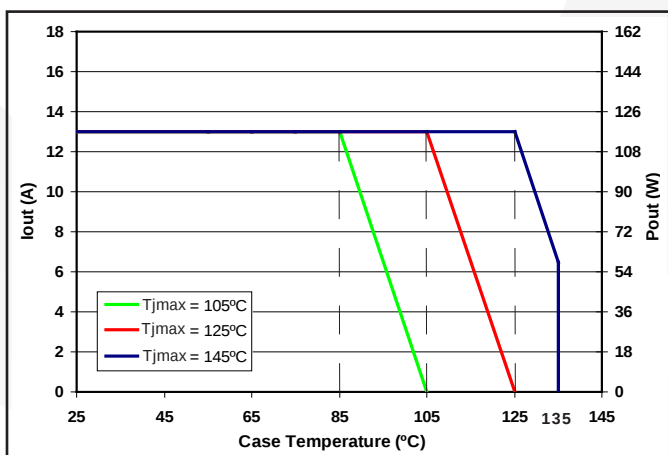
Figure 5: Output Current / Output Power derating curve as a function of T_{CASE} and the Maximum desired power MOSFET junction temperature. V_{in} = 270\text{V}
