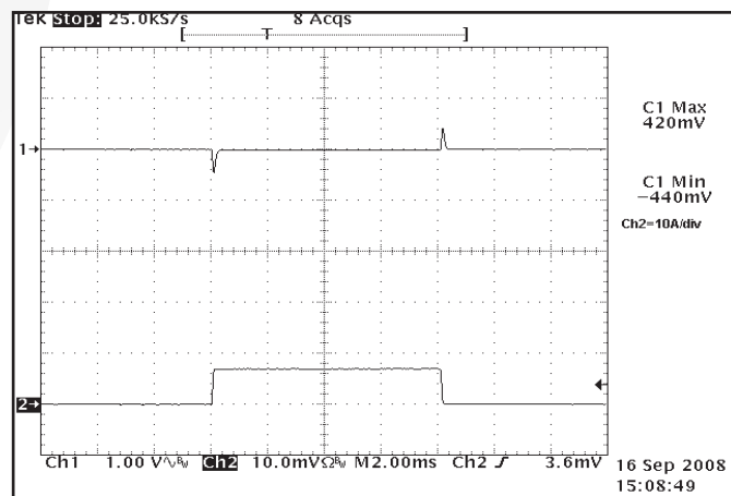
Figure 12: Output voltage response to step-change in load current 0%-50%-0% of I_{out} (max). Load cap: 1 \mu F ceramic cap and 10 \mu F, 100 m \Omega ESR tantalum cap. Ch 1: V_{out} (1V/div). Ch 2: I_{out} (10 A/div).
