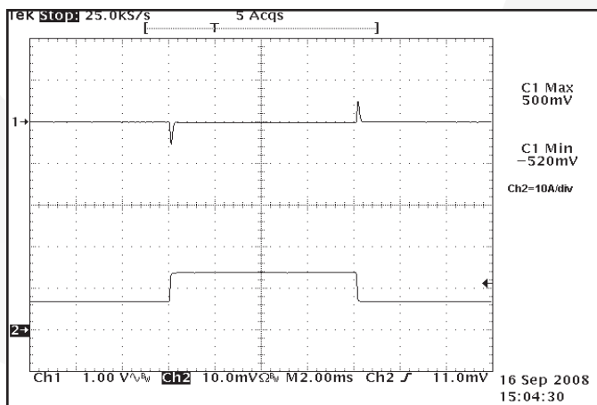
Figure 11: Output voltage response to step-change in load current 50%-100%-50% of I_{out} (max). Load cap: 1 \mu F ceramic cap and 10 \mu F, 100 m \Omega ESR tantalum cap. Ch 1: V_{out} (1V/div). Ch 2: I_{out} (10 A/div).
