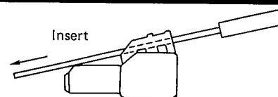
Fig. 1 IDC crimp
