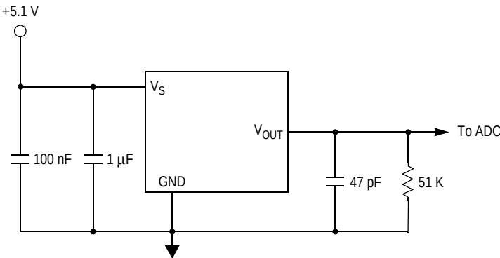
Figure 4. Typical application circuit (output source current operation)
