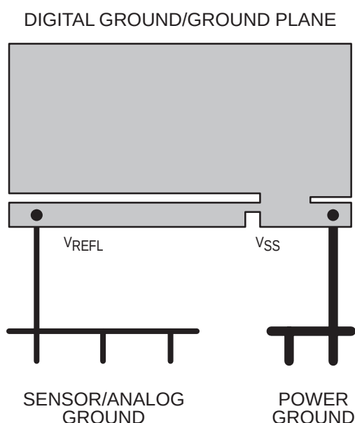
Figure 9. Ground Partitioning
