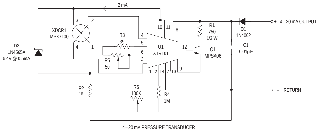
Figure 2. Schematic Diagram
