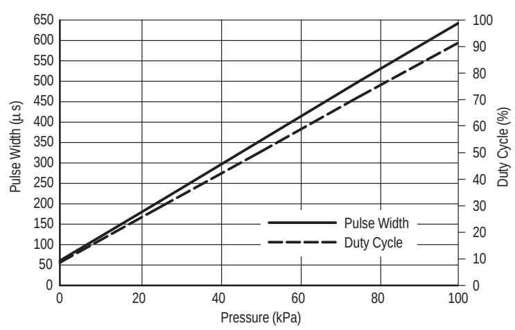
Figure 6. PWM Output Pressure Sensor Linearity Data
