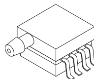
MPXV5050GP CASE 1369
