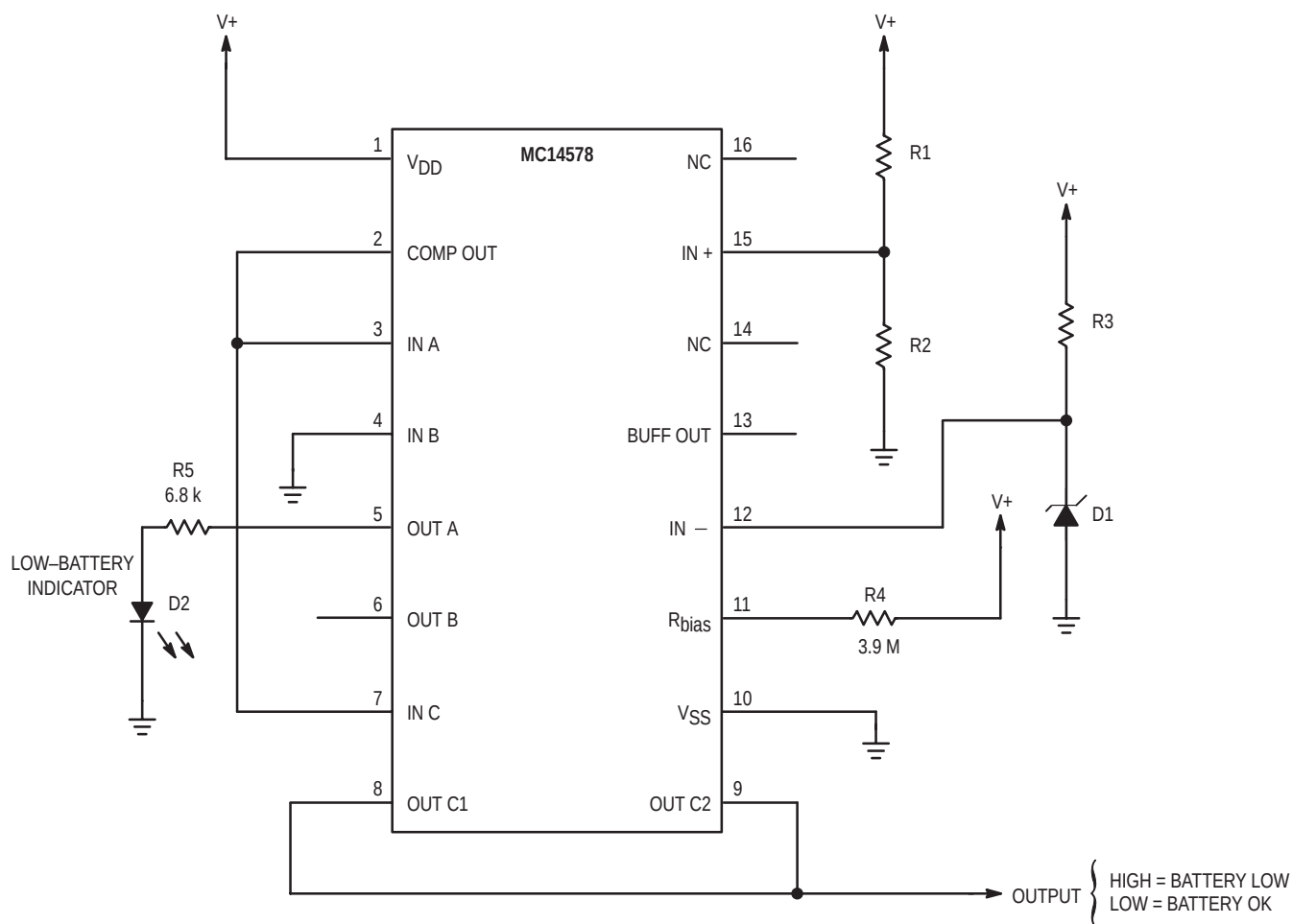
Figure 1. Low-Battery Detector
