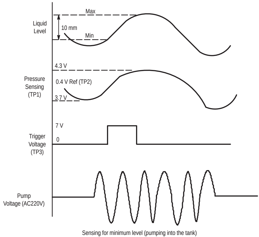
Figure 5. Functional Diagram
