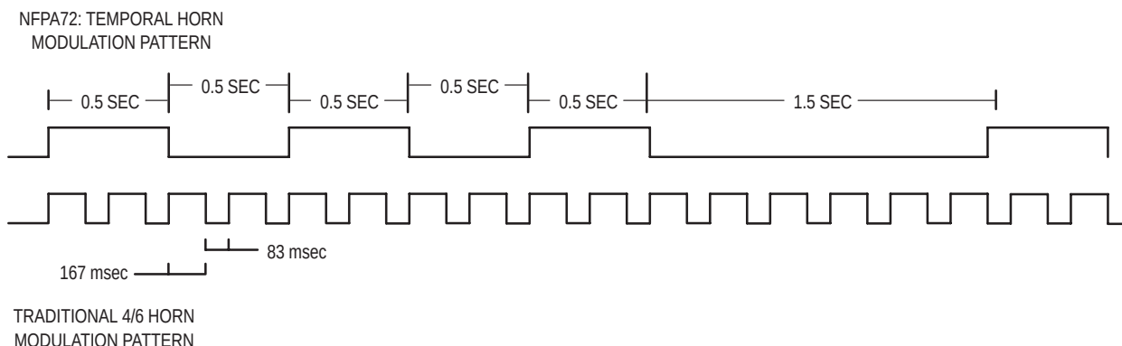
Figure 7. Horn Modulation
