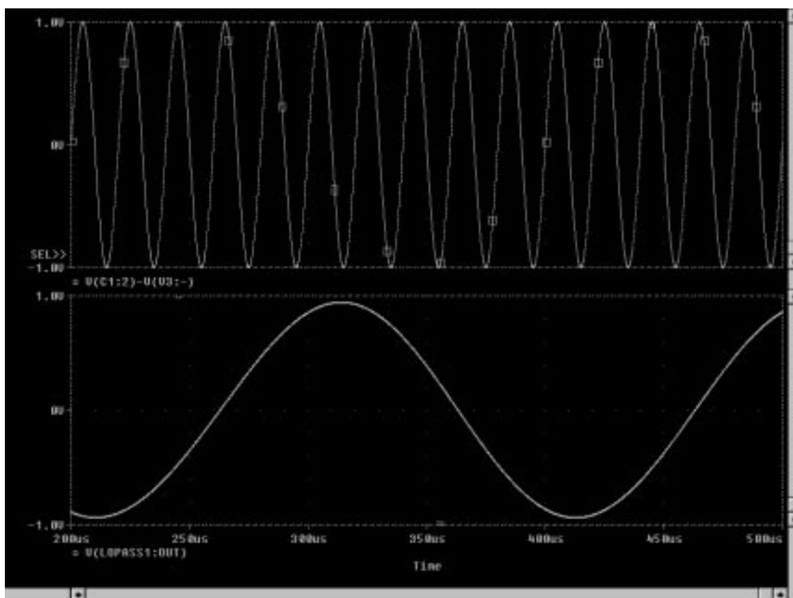
Figure 1. Aliased Signals
