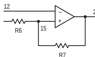
Figure 2. Adding Hysteresis
