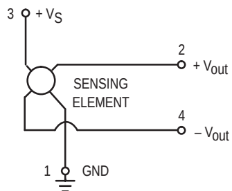
Figure 1. Uncompensated Pressure Sensor Schematic
