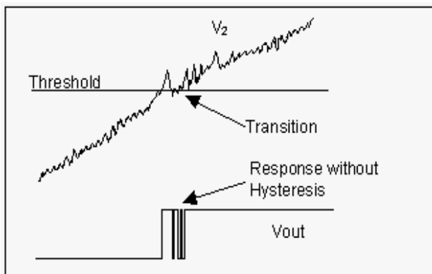
Figure 5a. Output Transition without Hysteresis
