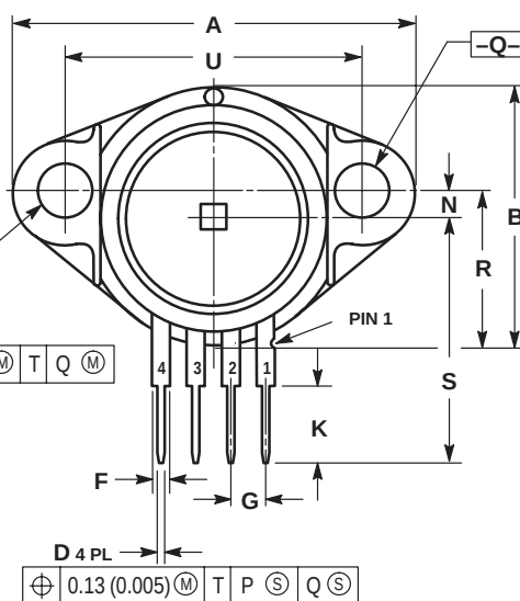
CASE 344F-01 ISSUE B
