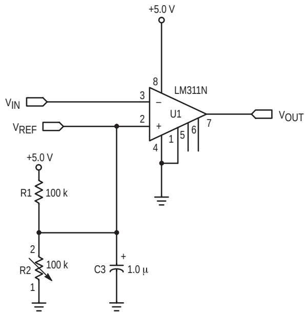
Figure 3. Comparator Circuitry
