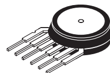
MPX4200A CASE 867
