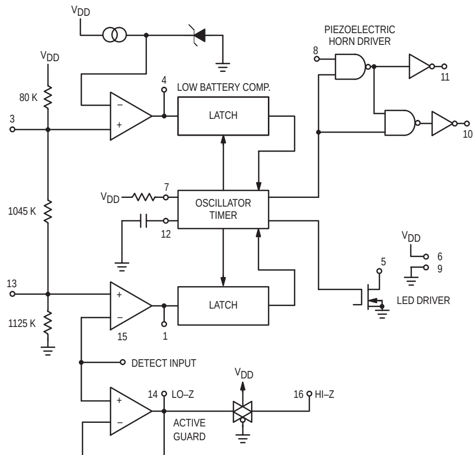
Figure 1. Block Diagram
