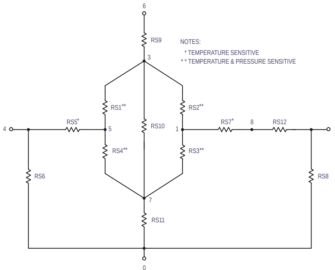
Figure 2. MPX2000 Series PSPICE Compound Coefficient Model
