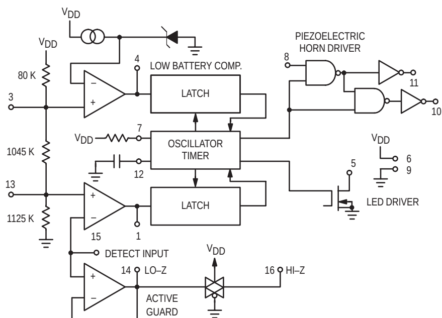
Figure 1. Block Diagram
