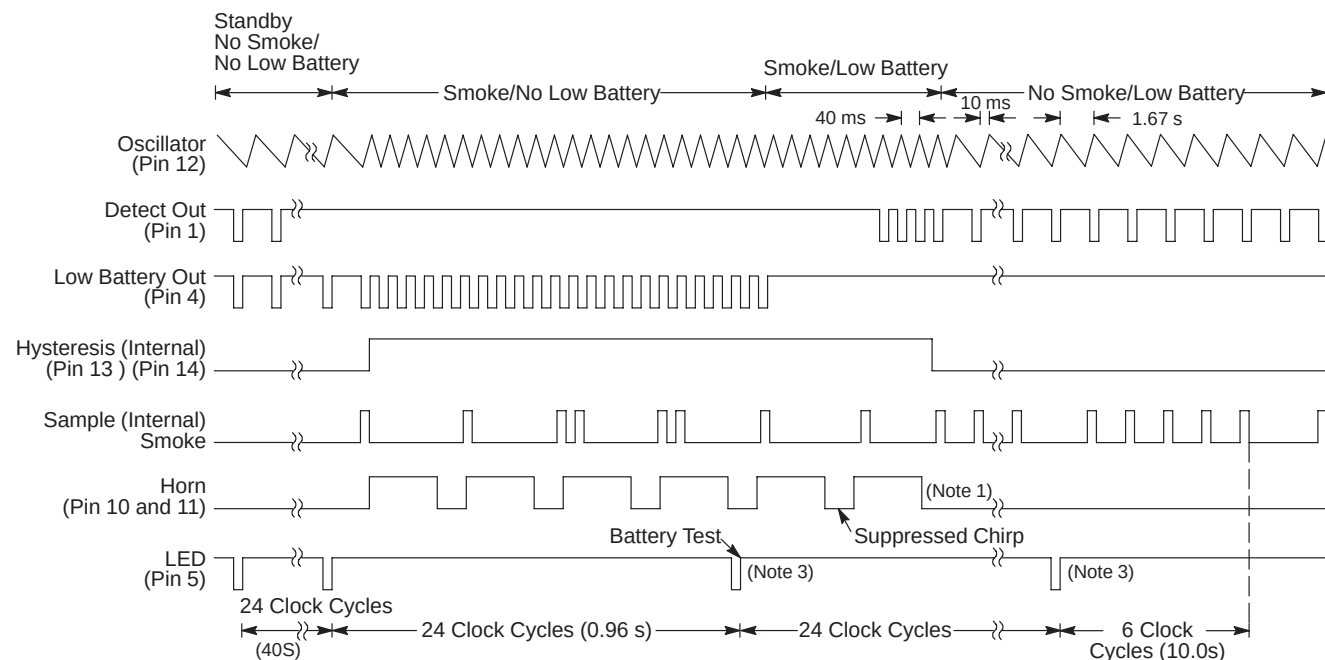
Figure 6. Timing Diagram
