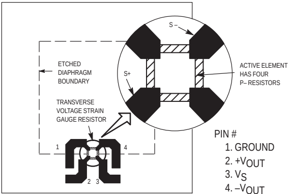
Figure 3a. Localized Sensing Element
