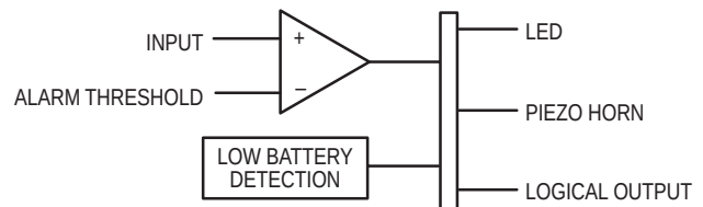
Figure 1. Alarm IC Concept
