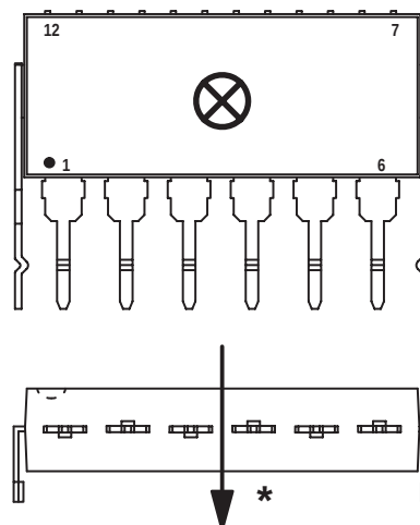
WINGBACK PACKAGE
