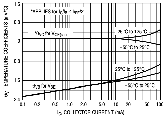
Figure 32. Temperature Coefficients
