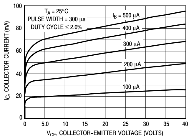
Figure 10. Collector Characteristics
