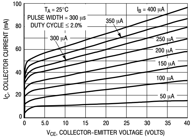
Figure 30. Collector Characteristics
