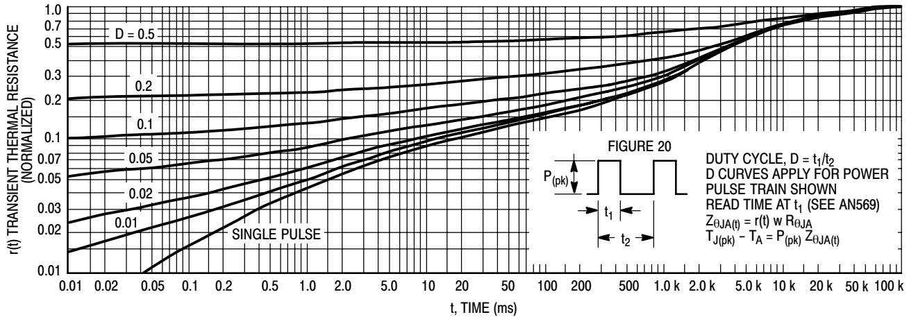
Figure 19. Thermal Response
