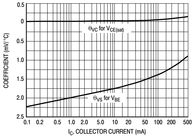
Figure 17. Temperature Coefficients
