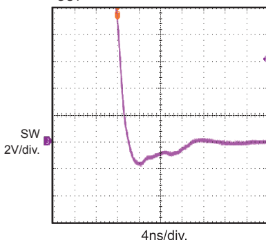
Dead Time (off)
