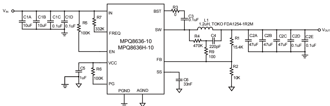
MPQ8636-10, MPQ8636H-10, V_{OUT}=1.5V , I_{OUT}=1A-10A , f_{SW}=500kHz
