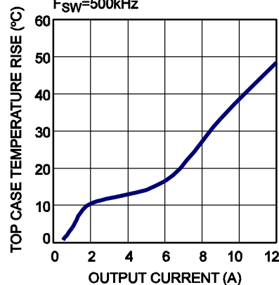
Case Temperature Rise vs. Output Current F_{SW} = 500kHz
