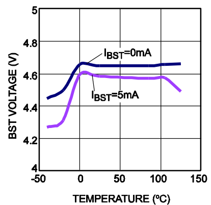
BST Voltage vs. Temperature
