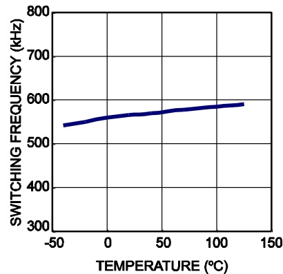
Switching Frequency vs. Temperature I_{OUT} = 6A , R_{FREQ} = 332k\Omega
