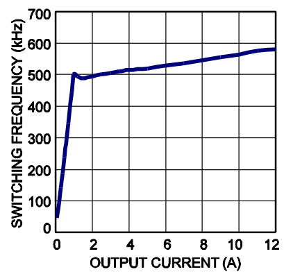
Switching Frequency vs. Output Current R_{FREQ} = 332k\Omega
