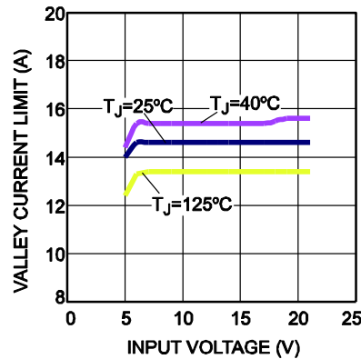
Valley Current Limit vs. Input Voltage
