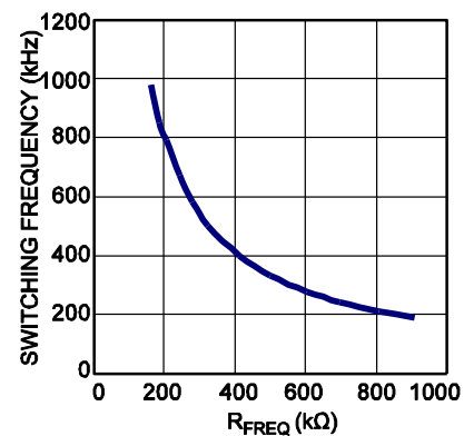
Switching Frequency vs. R_{FREQ}
