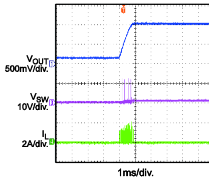
Thermal Recovery
