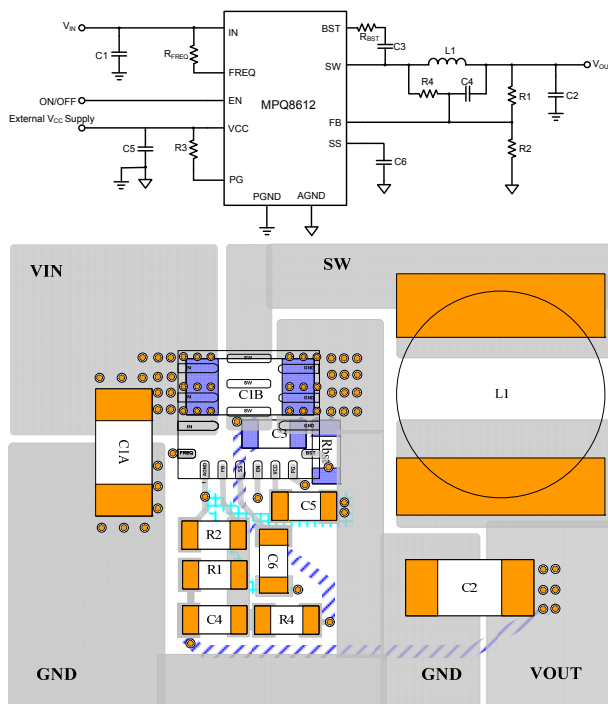
Figure 16—PCB LAYOUT
