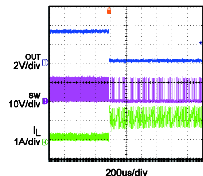
Short Circuit Entry I_{OUT}=0.1A to Short
