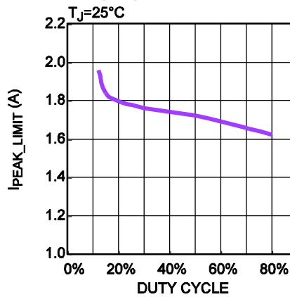
Current Limit vs. Duty Cycle
