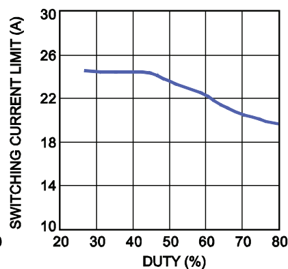
Internal Current Limit vs. Duty
