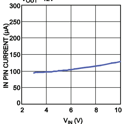
IN Quiescent Current vs. Input Voltage
