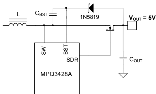
Figure 3: BST Charger for Low-Output Application
