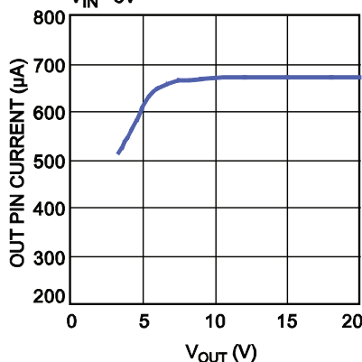
OUT Quiescent Current vs. Output Voltage
