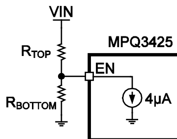
Figure 2: UVLO Hysteresis
