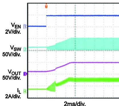
EN Start-Up V_{IN} = 10V , I_{OUT} = 0.4A
