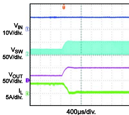
Over-Current Recovery V_{IN} = 10V , I_{OUT} = 0.1A to 2A
