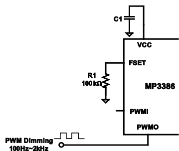
Figure 5— Direct PWM Dimming with Negative Logic
