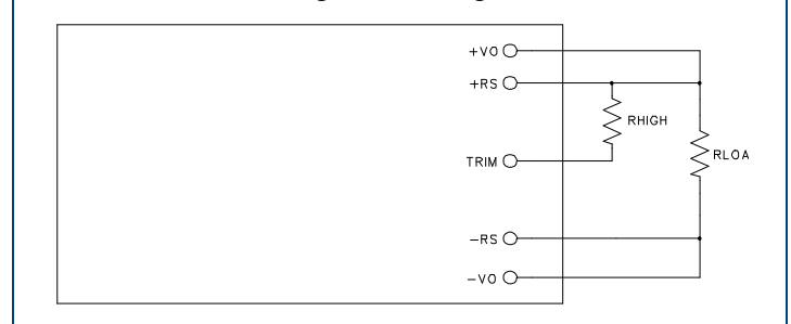
Figure 4: Trim High
