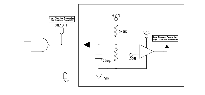
Figure 1: Active High
