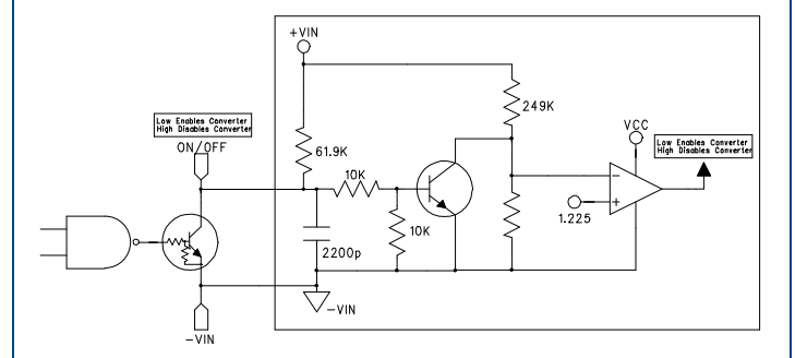
Figure 2: Active Low
