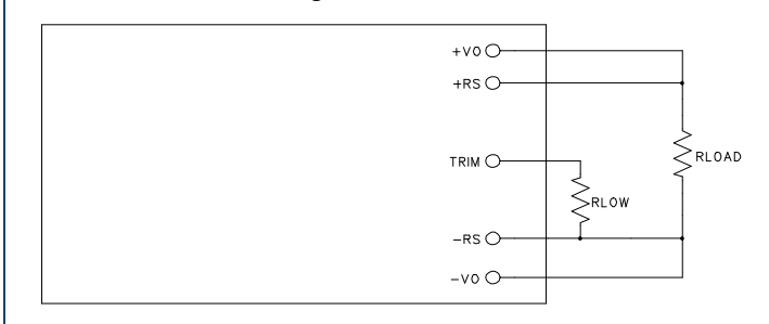
Figure 3: Trim Low
