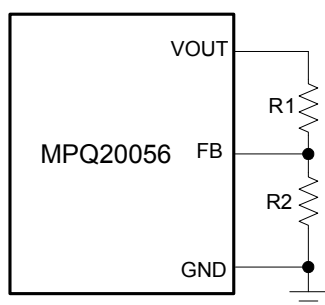
Figure 3: Setting the Output Voltage
