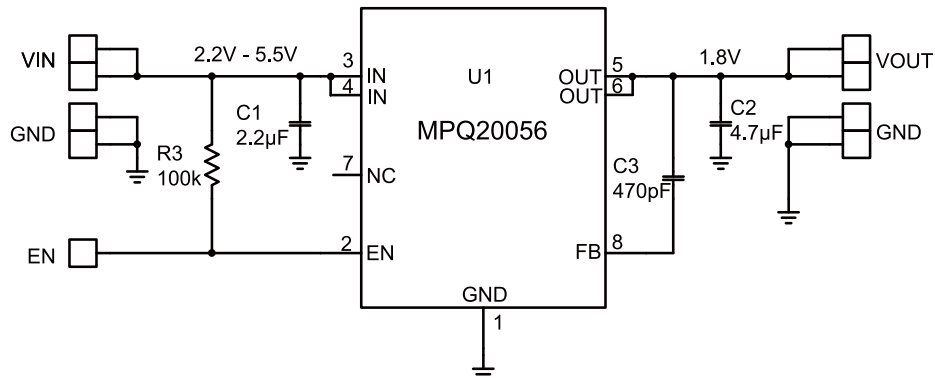
Figure 4: 1.8V Fixed Output Application (QFN-8L)
