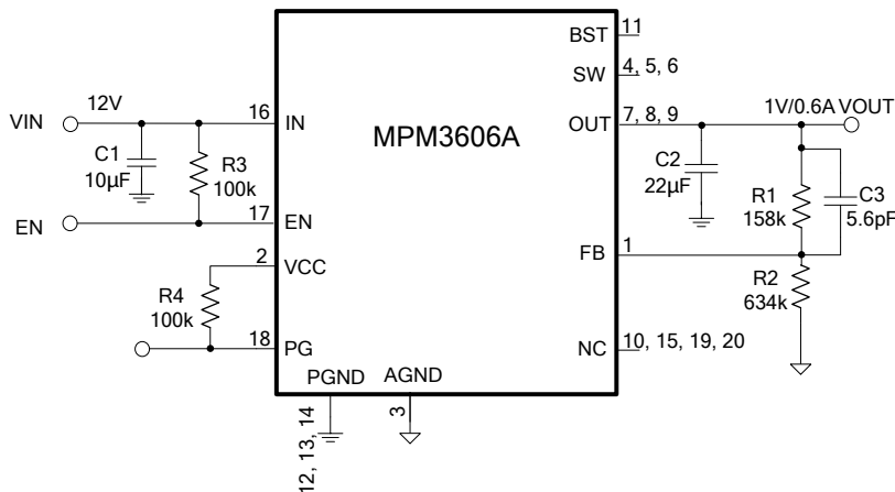
Figure 15: V_o=1V , I_o=0.6A
