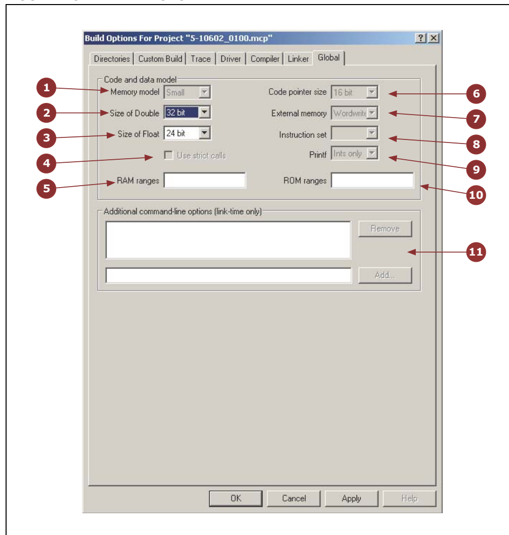
FIGURE 4-8: THE GLOBAL TAB
