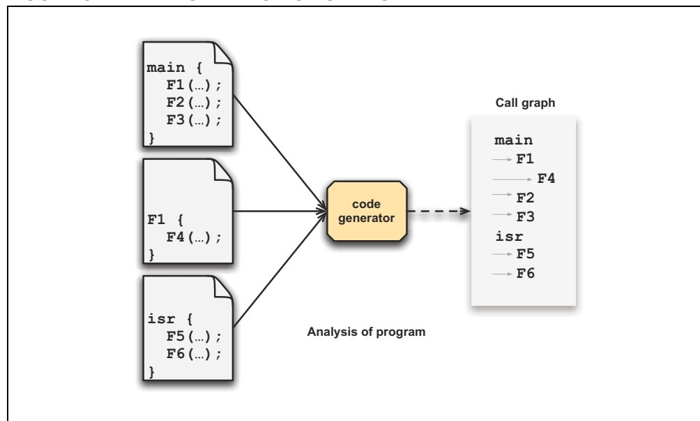
FIGURE 5-2: FORMATION OF CALL GRAPH
