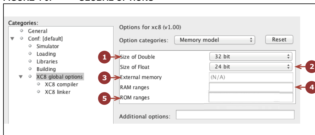
FIGURE 4-9: GLOBAL OPTIONS
