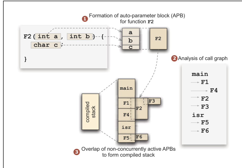
FIGURE 5-3: FORMATION OF THE COMPILED STACK
