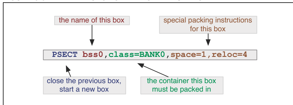
FIGURE 5-6: THE SECTION DIRECTIVE AS A BOX LABEL
