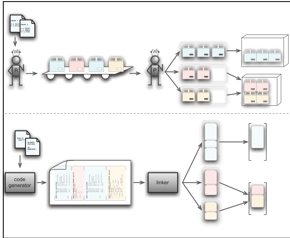
FIGURE 5-4: THE WAREHOUSE AND COMPILER SIDE BY SIDE
