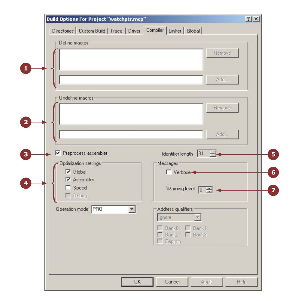
FIGURE 4-6: THE COMPILER TAB
