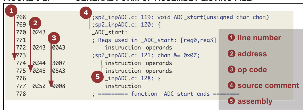
FIGURE 6-1: GENERAL FORM OF ASSEMBLY LISTING FILE
