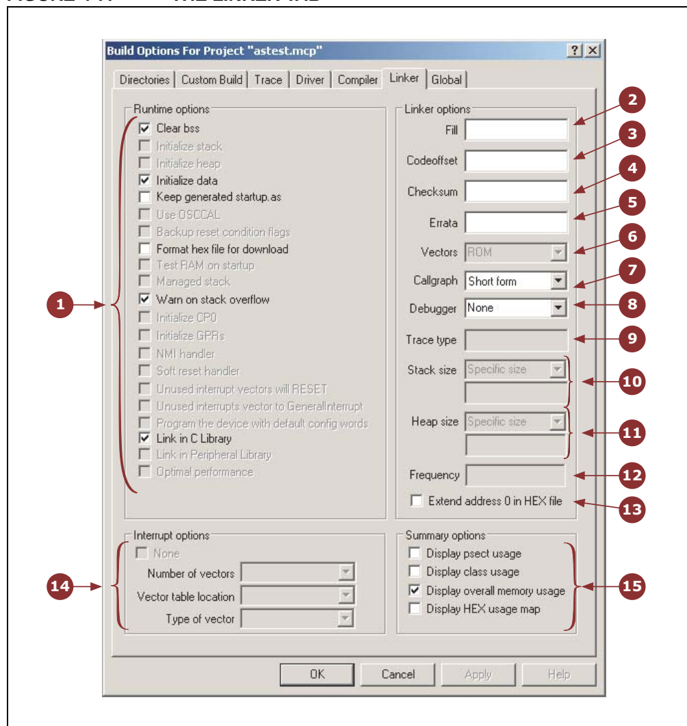
FIGURE 4-7: THE LINKER TAB
