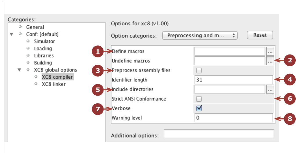
FIGURE 4-10: PREPROCESSING AND MESSAGES OPTIONS
