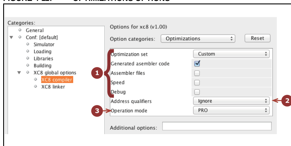
FIGURE 4-11: OPTIMIZATIONS OPTIONS
