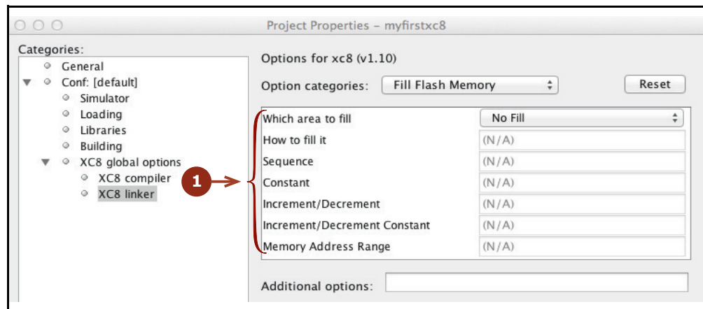
FIGURE 4-11: FILL FLASH MEMORY OPTIONS
