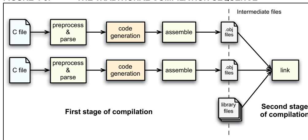
FIGURE 4-3: THE TRADITIONAL COMPILATION SEQUENCE
