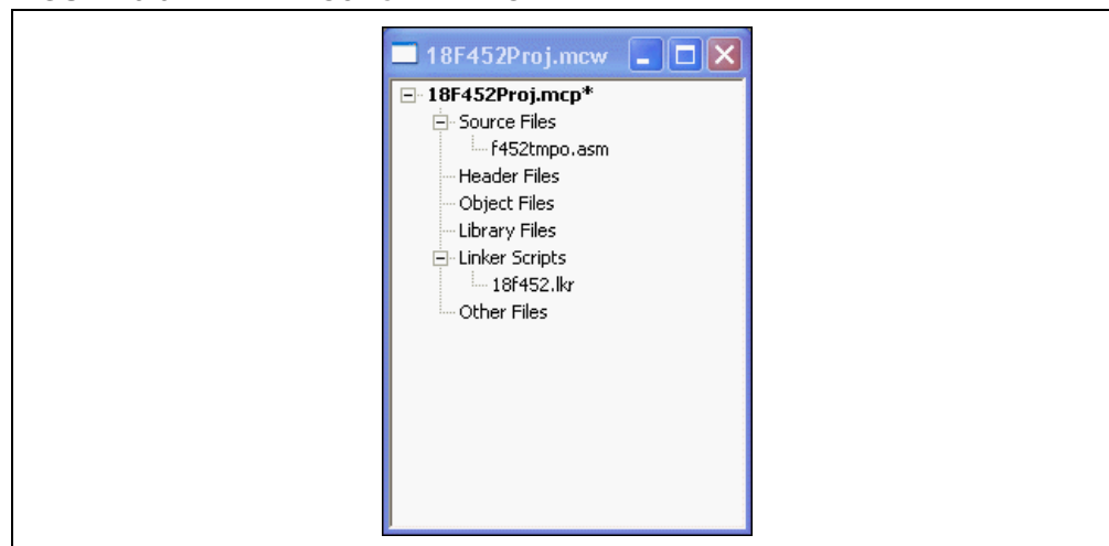
FIGURE 3-9: PROJECT WINDOW
