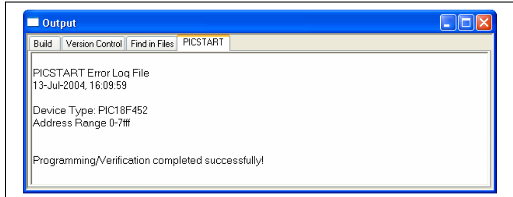
FIGURE 3-17: PROGRAMMING RESULTS
