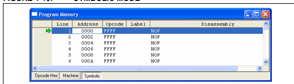
FIGURE 4-10: SYMBOLIC MODE
