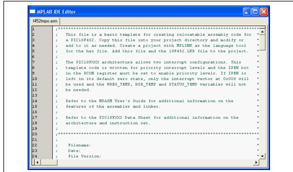
FIGURE 3-11: TEMPLATE FILE
