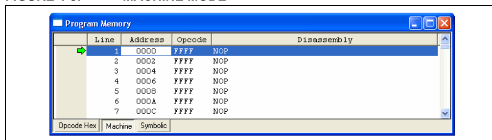
FIGURE 4-8: MACHINE MODE
