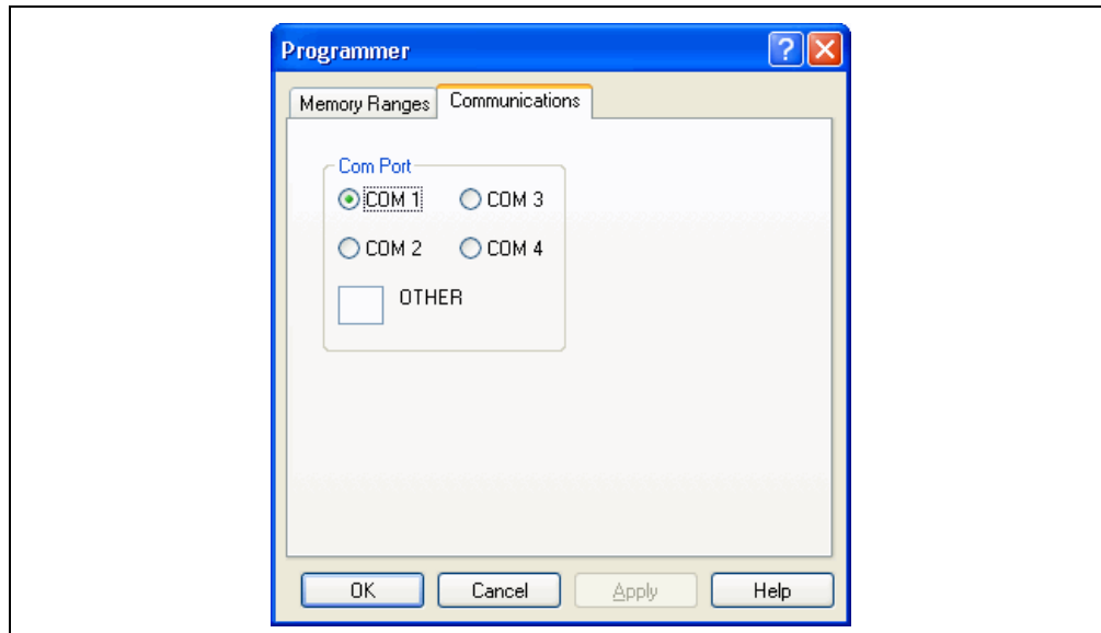
FIGURE 5-9: COMMUNICATIONS TAB
