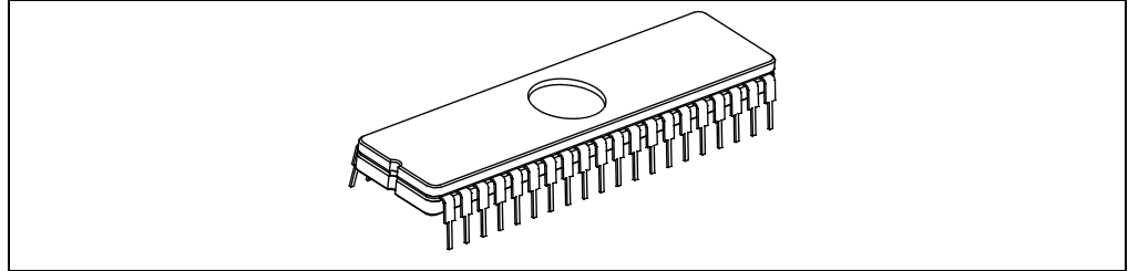
FIGURE 4-21: WINDOWED DEVICE
