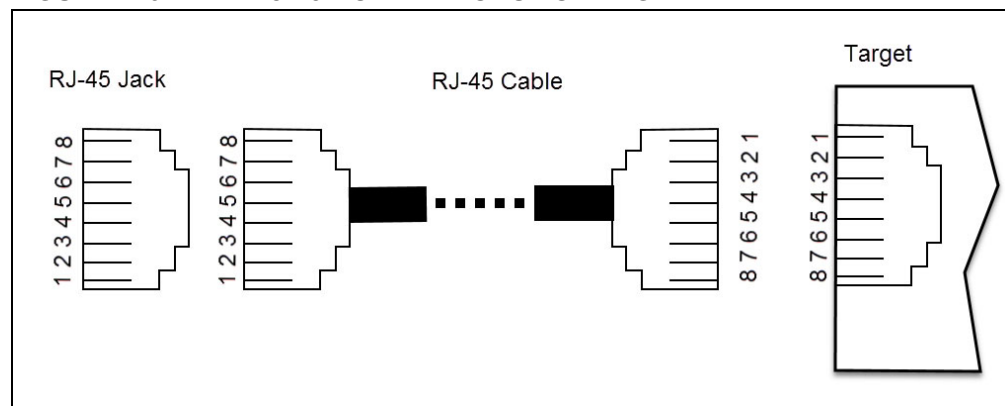
FIGURE B-6: RJ-45 CONNECTIONS TO TARGET
