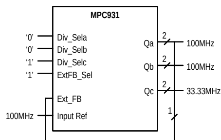
Figure 10. "Zero" Delay Divide by 3 (50% Duty Cycle)
