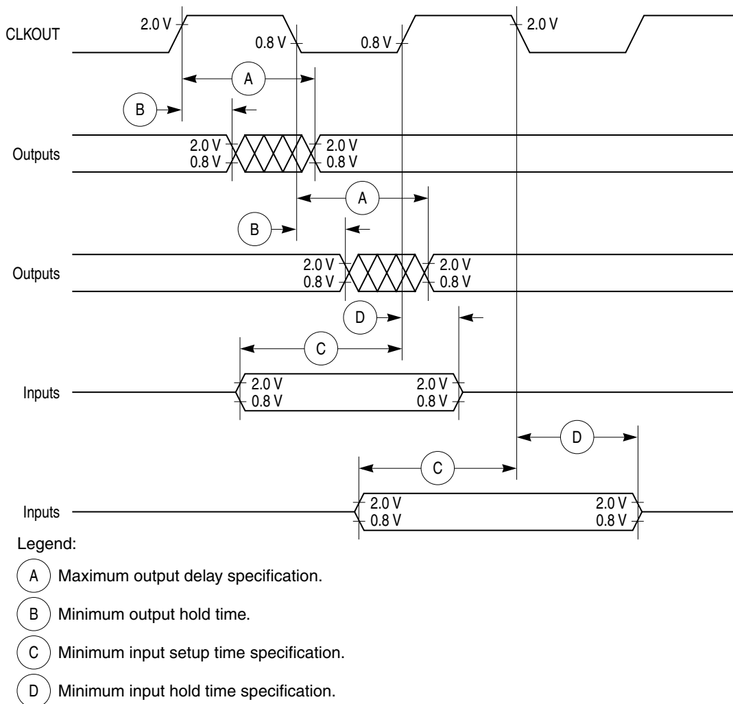
Figure 4. Control Timing
