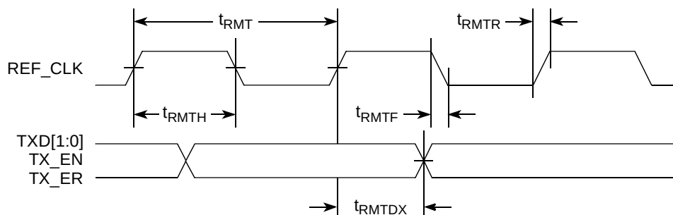
Figure 16. RMII Transmit AC Timing Diagram
