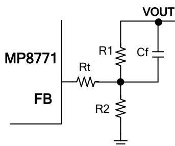
Figure 7: Feedback Network
