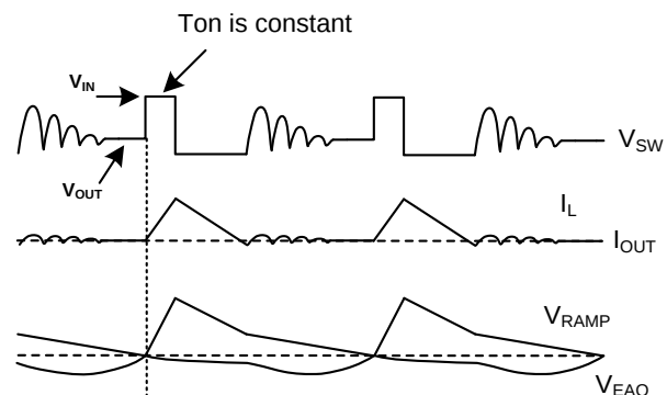
Figure 4: Light-Load Operation
