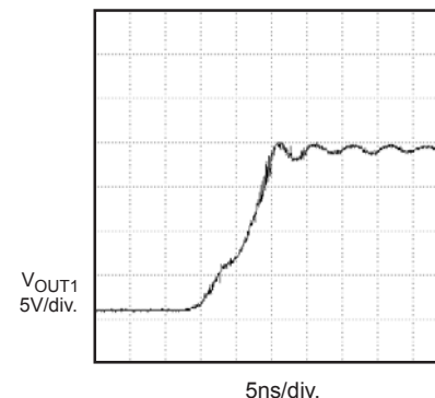
Output Rise-Time
