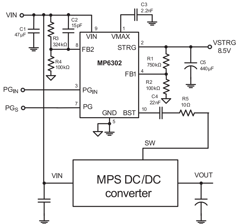
Figure 6—MP6302 Application Circuit
