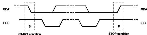
Figure 14: START and STOP Conditions
