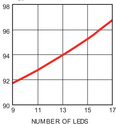
Efficiency vs. LED number
