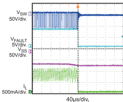
Open LED Load @ Working
