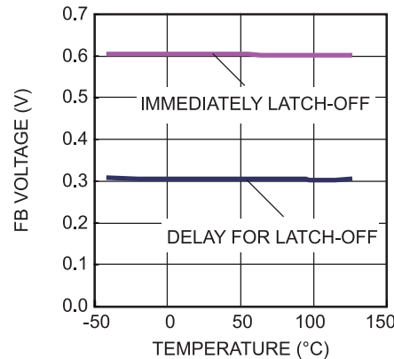
SLP Threshold vs. T_J
