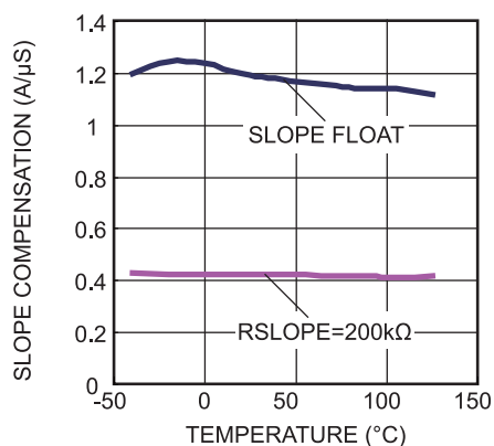
Slope Compensation vs. T_J
