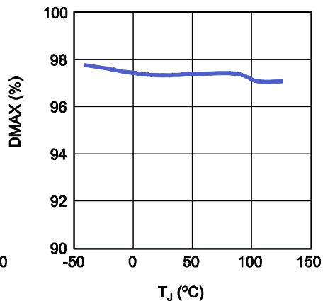
Maximum Duty vs. T_J R_T=499k\Omega
