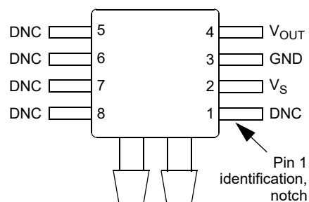
Pinout
