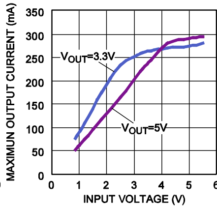
Maximum Output Current vs. Input Voltage (6)
