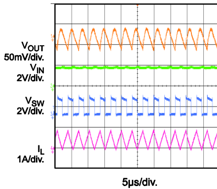
Output Ripple I_{OUT}=0.2A
