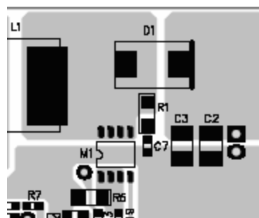
Figure 4—Layout Consideration
