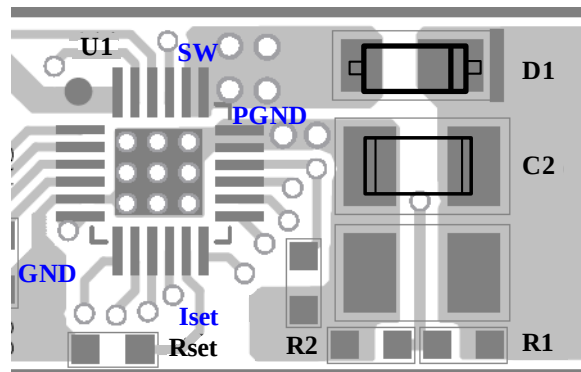
Figure 7—Layout Consideration
