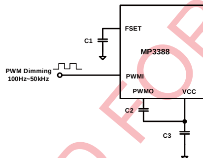
Figure 3—PWM Dimming
