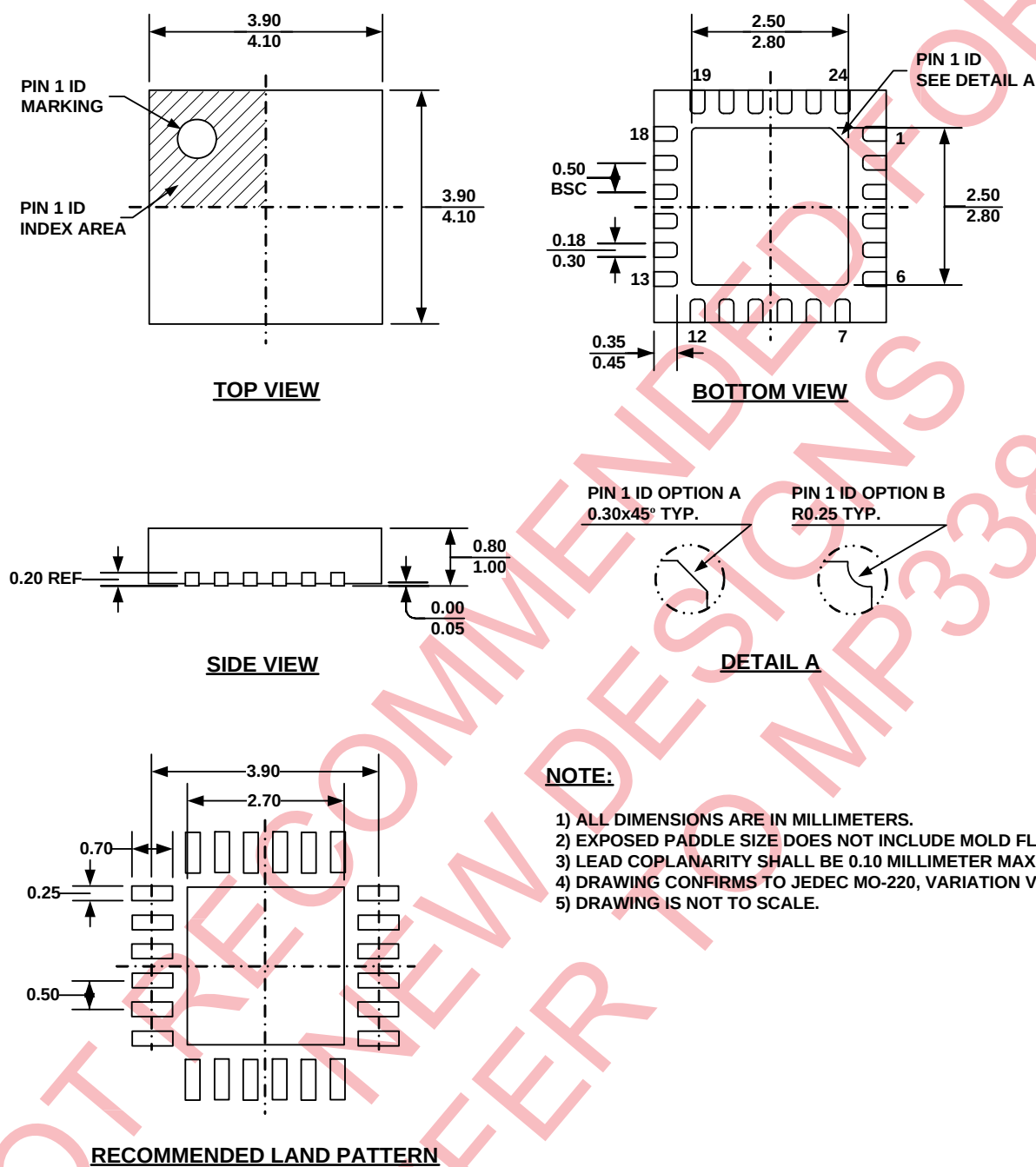
QFN24 (4mm x 4mm)
