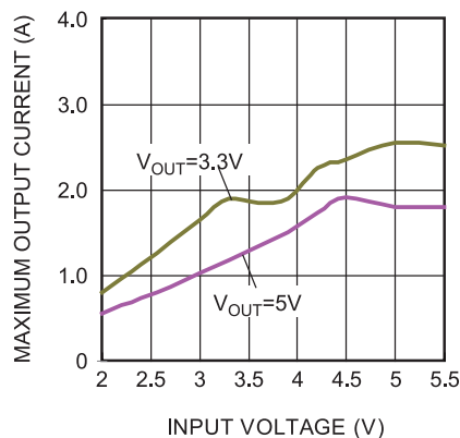
Output Current Capability vs. Input (6)
