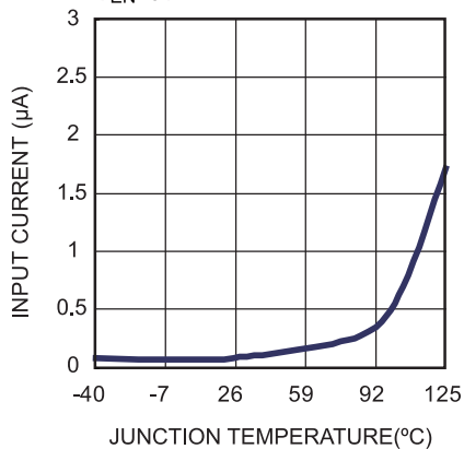
Disabled Supply Current vs. Temperature V_{EN}=0V
