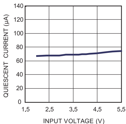
Quiescent Current V_{FB}=0.65V
