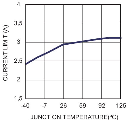
Primary Current Limit vs. Temperature
