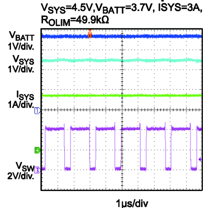
Boost Mode CC Operation
