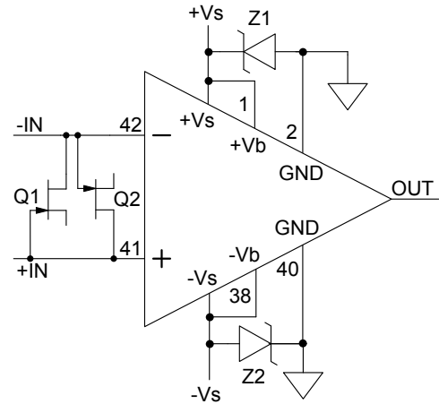
FIGURE 1: OVERVOLTAGE PROTECTION
