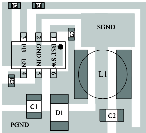
Figure 2—PCB Layout
