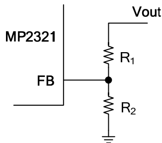
Figure 8: Feedback Network
