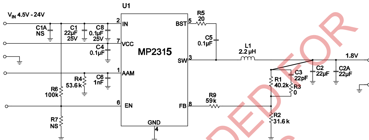
Figure 12: V_o=1.8V , I_o=3A
