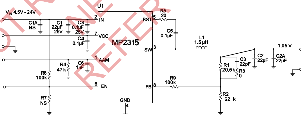
Figure 14: V_o=1.05V , I_o=3A
