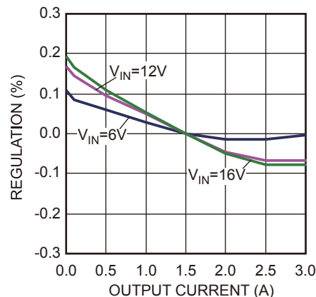
Load Regulation V_{IN} = 6V-16V , I_{OUT} = 0A-3A
