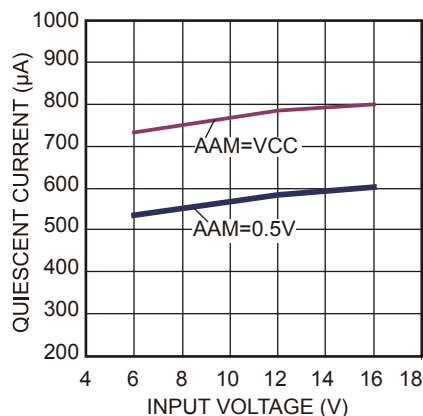
Quiescent Current vs. Input Voltage V_{IN} = 6V-16V , V_{FB} = 1V
