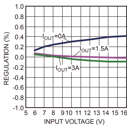
Line Regulation V_{IN} = 6V-16V
