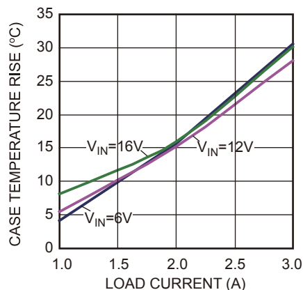
Case Temperature Rise vs. Output Current I_{OUT} = 0A-3A
