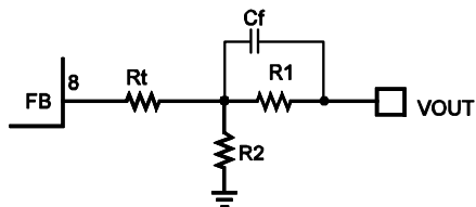
Figure 3: T-Type Network
