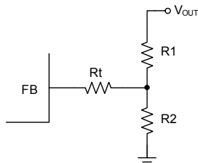
Figure 2—Feedback Network
