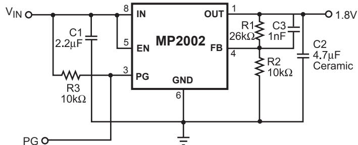
Figure 3—Typical Application Circuit with Fix Pinout
