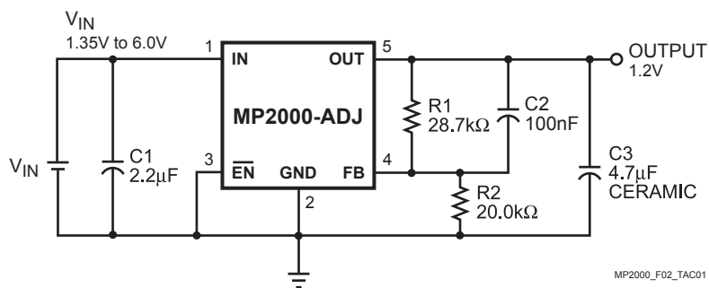
Figure 3—Typical Application Circuit with V_{OUT} = 1.2V
