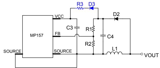
Figure 9: Auxiliary V_{CC} Supply Circuit
