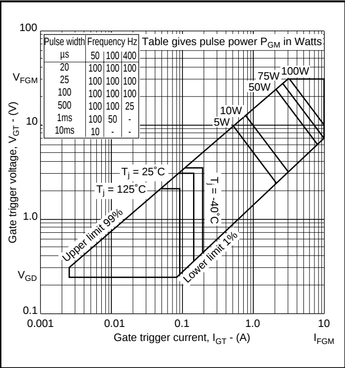
Fig. 5 Gate characteristics
